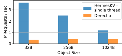
Figure 8. Comparison to Derecho. [Uniform traffic, 5 nodes, write-only]
